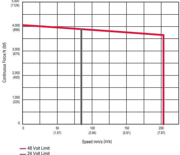
GTX080 - 02 5.08 mm (0.2 in) Screw Lead
